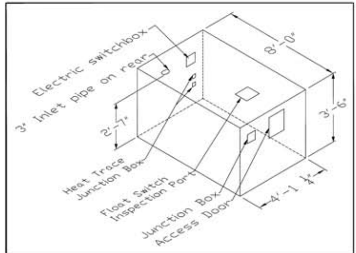
Sewage Tank as Supplied
