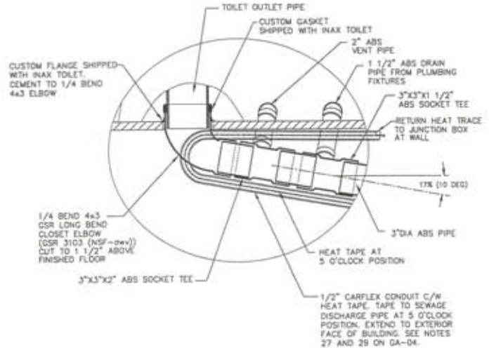
Detail of Typical Discharge Piping
